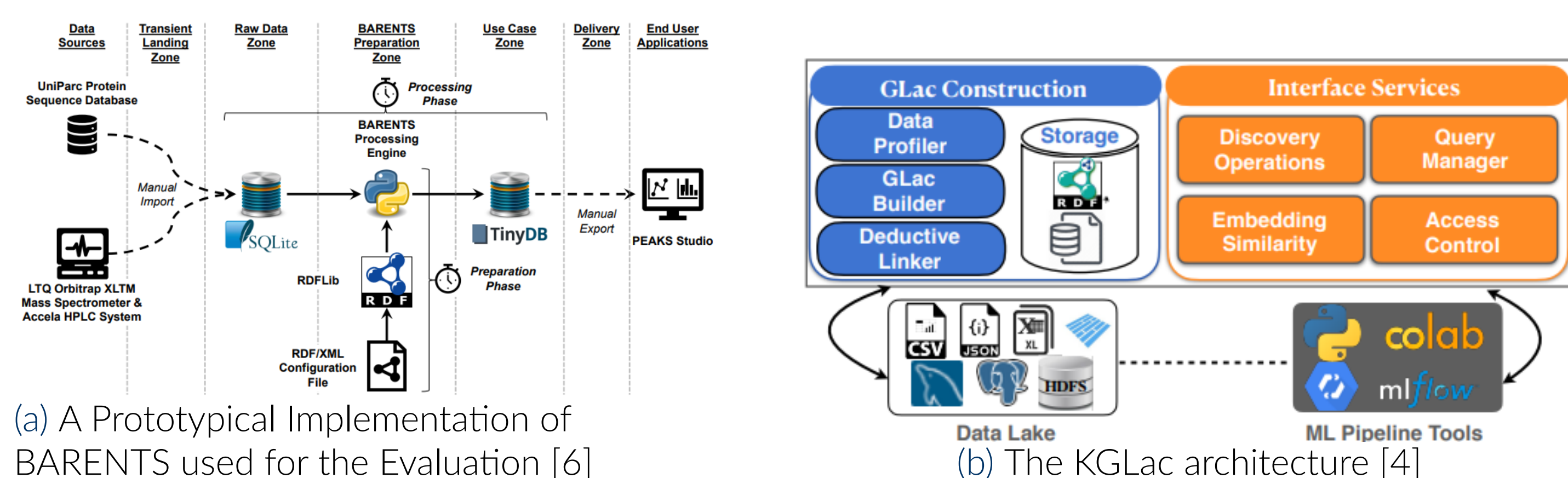
Figure 5. Two Context-aware Data Discovery Platforms
