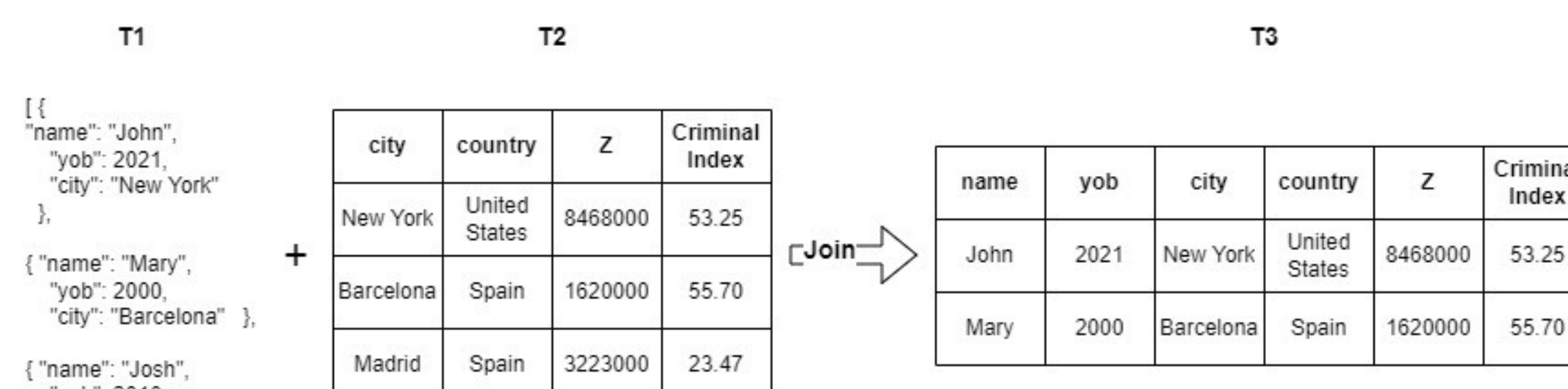
Figure 3. Join Operation with Heterogeneous Data in the Data Lake
