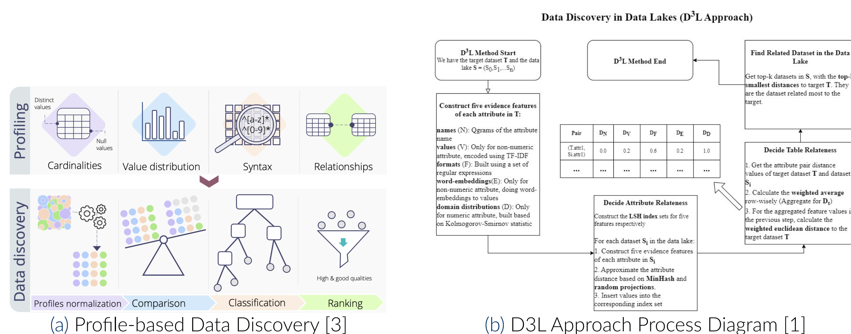
Figure 4. Data Discovery Methods
