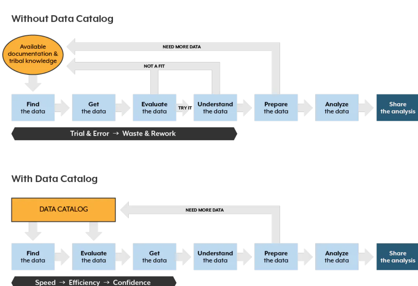
(b) Data discovery with & without data catalog [7]
